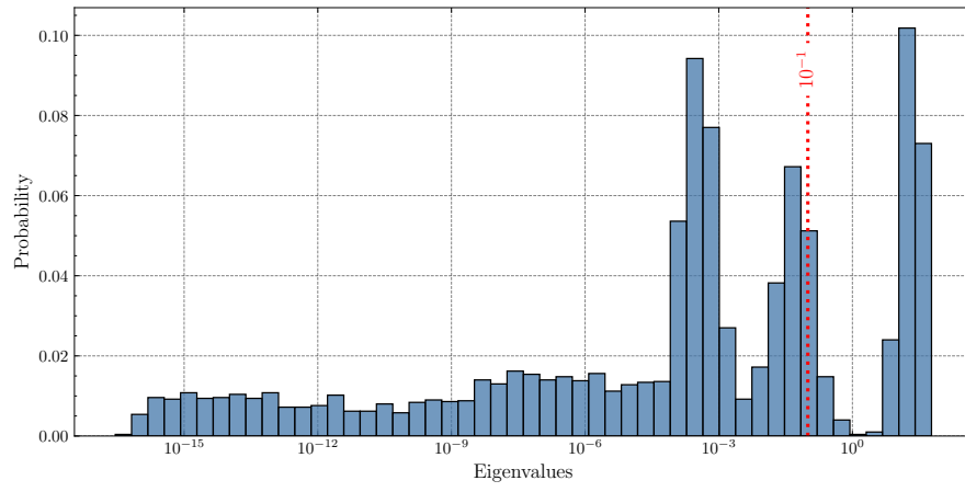
Figure 4.2: Probability mass function of the eigenvalues across all calculated empirical observability gramians
