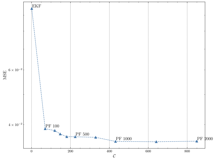
Figure 4.3: Comparison of the computational complexity and error across all estimators
