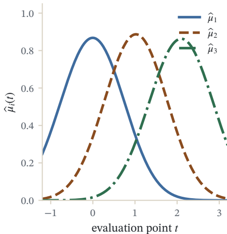
2 One mean embedding per bag
