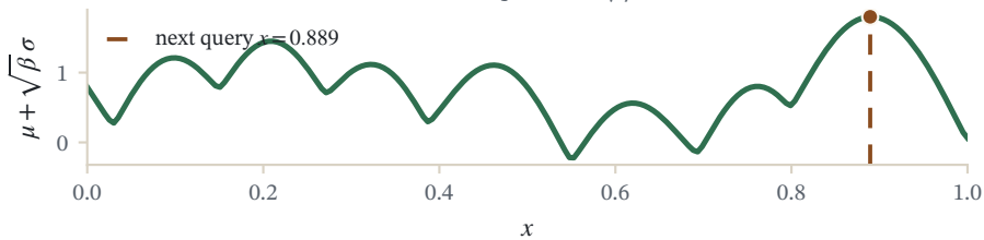
GP-UCB acquisition, \sqrt{\beta} = 2
