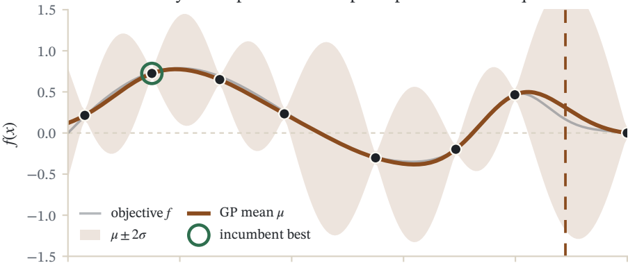
The Bayesian optimization loop: GP posterior after 8 queries
