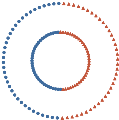
Euclidean K-means
