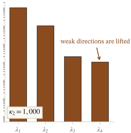
After adding \lambda I , \lambda = 0.01
