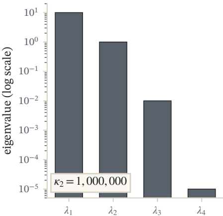
Raw Gram spectrum
