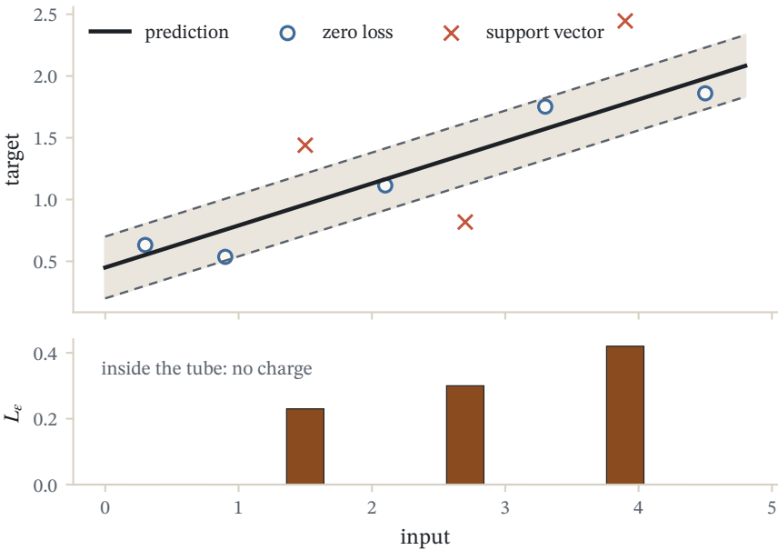
An \varepsilon -tube with \varepsilon=0.25
