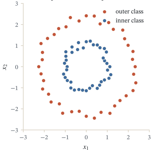
In the plane: no line separates them
