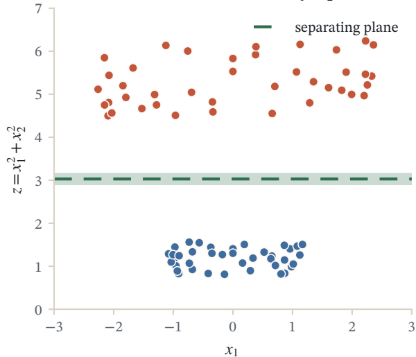
Lifted by \phi(x) = (x_1, x_2, x_1^2 + x_2^2)
