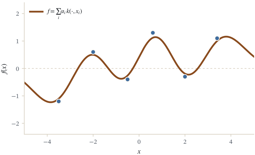
Kernel ridge, Gaussian kernel, bandwidth 1, \lambda = 10^{-2}
