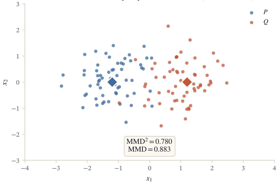
Maximum mean discrepancy, Gaussian kernel (bandwidth 1.2)
