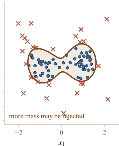
\nu = 0.3 : accepted 69%
