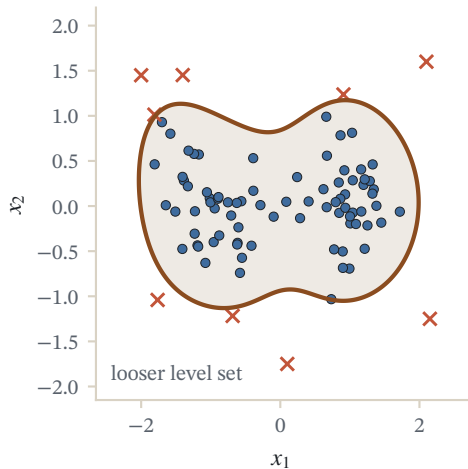
\nu = 0.1 : accepted 90%
