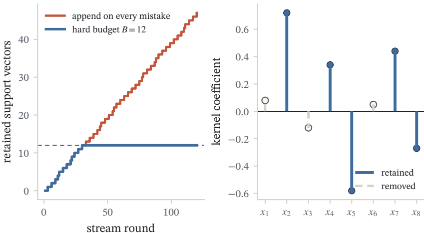
Prediction cost follows support-set size A cheap rule deletes small contributions
