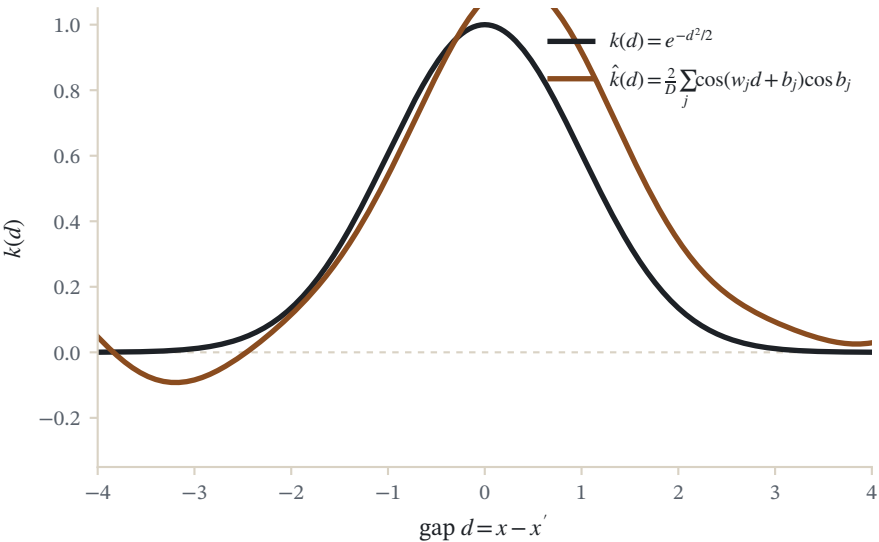
Random Fourier features, D = 20 -- RMSE = 0.143
