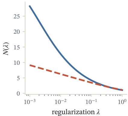
Effective dimension
