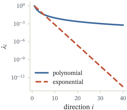
Spectral decay
