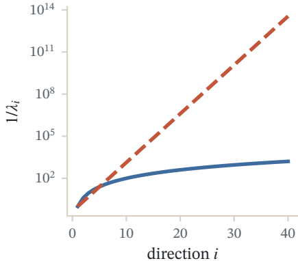
RKHS cost
