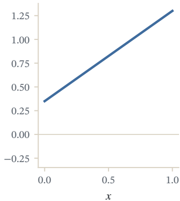
null-space trend
