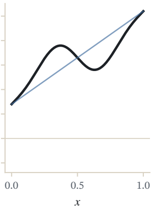
spline fit
