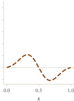
penalized bend
