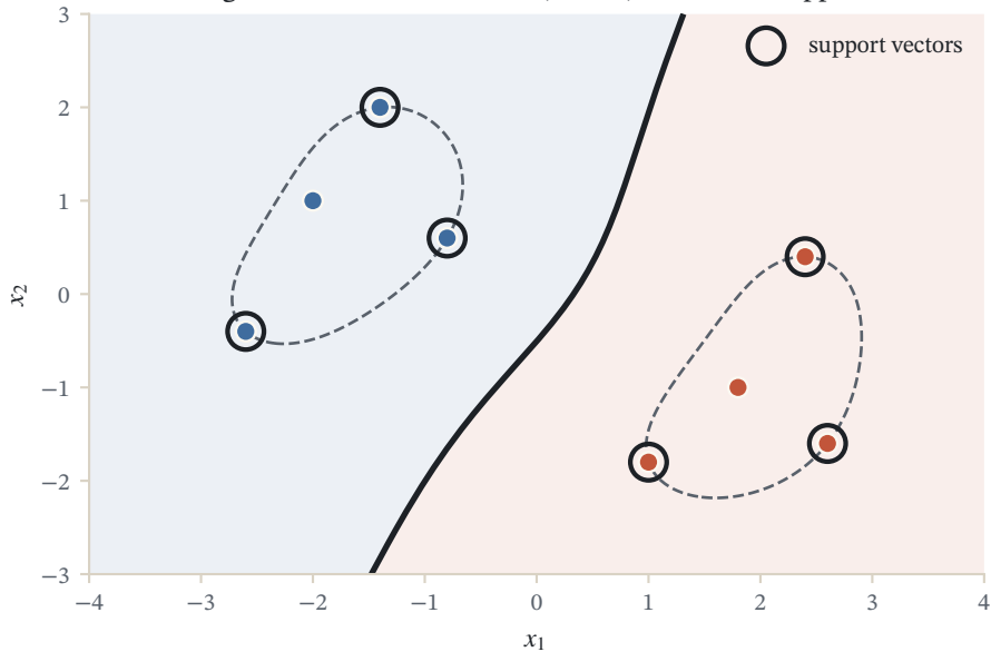
Max-margin SVM, Gaussian kernel (bw 1.2), C = 10 -- 6 support vectors
