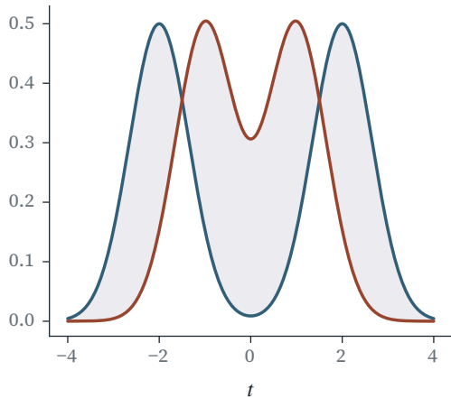
Gaussian kernel: distinct embeddings
