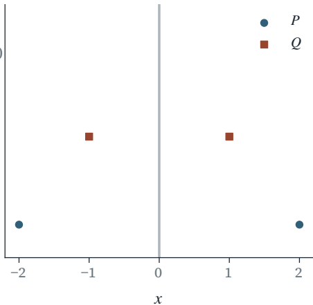
linear kernel: same mean
