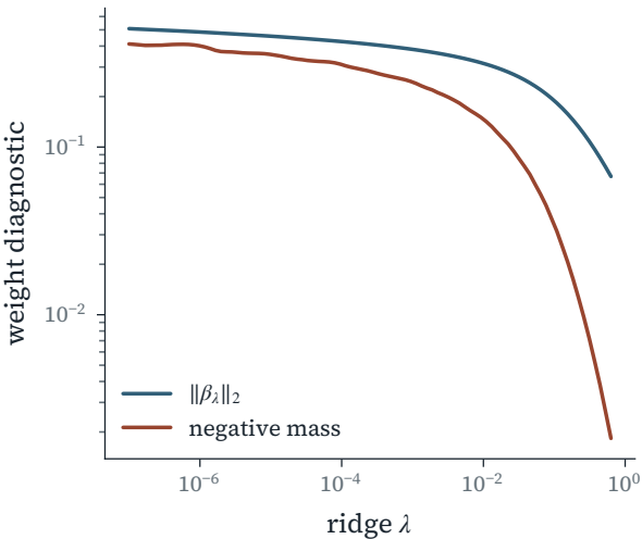
Regularization suppresses cancellation
