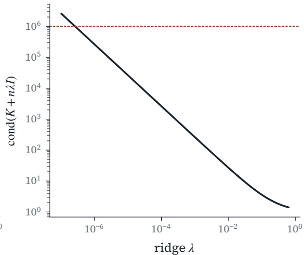
The spectral floor stabilizes the solve
