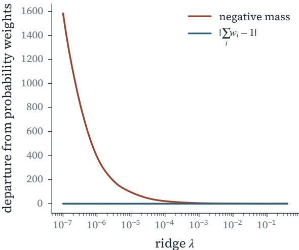
Coordinates need not form a simplex
