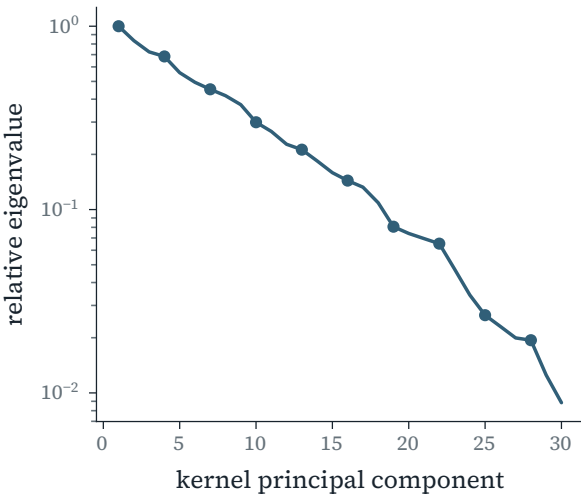
Centered Gram spectrum
