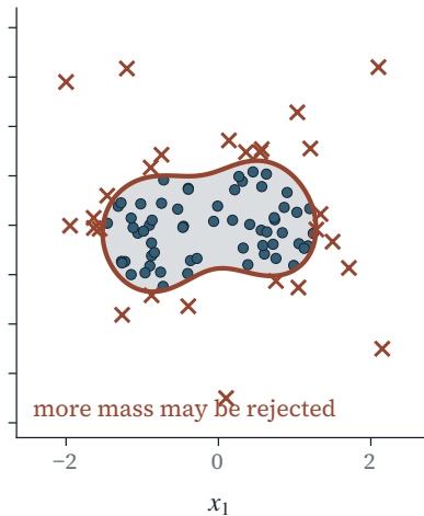
\nu = 0.3 : accepted 69%
