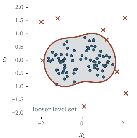
\nu = 0.1 : accepted 90%
