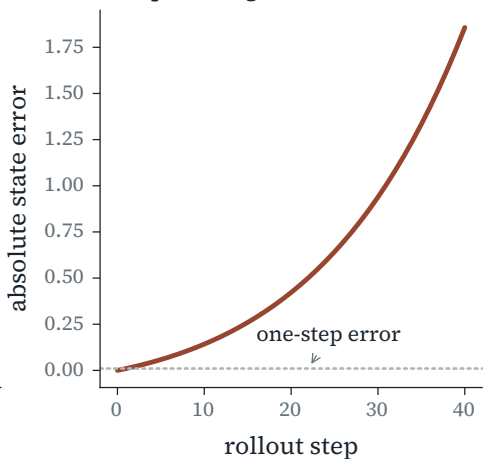
Compounding bias
