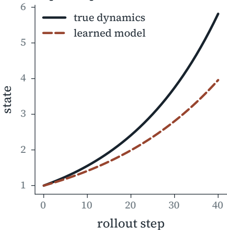
Repeated prediction
