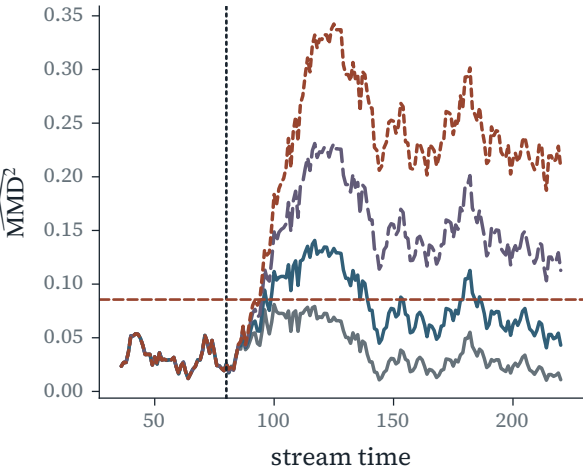
Sequential MMD after a mean shift
