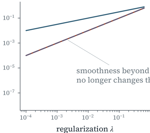
Tikhonov: qualification 1
