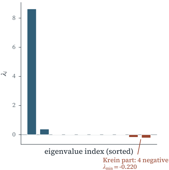
tanh similarity spectrum, S_{ij} = \tanh(ax_i x_j + b) , a = 1
