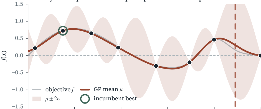
GP-UCB acquisition, \sqrt{\beta} = 2
