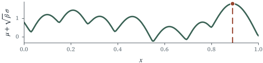
GP-UCB acquisition, \sqrt{\beta} = 2
