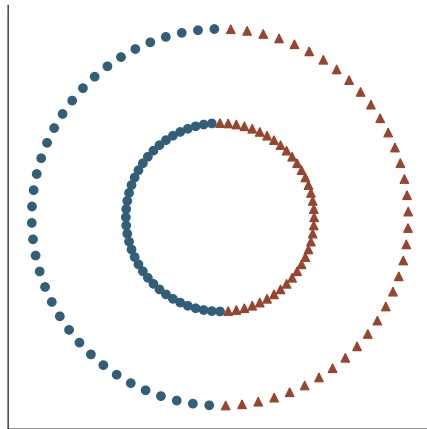
Euclidean K-means
