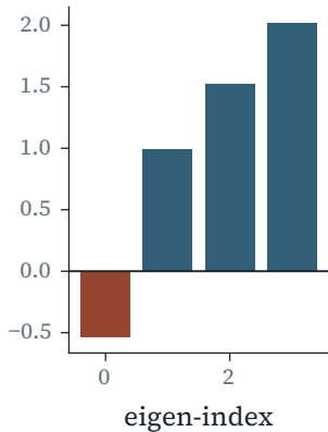
Signed spectrum
