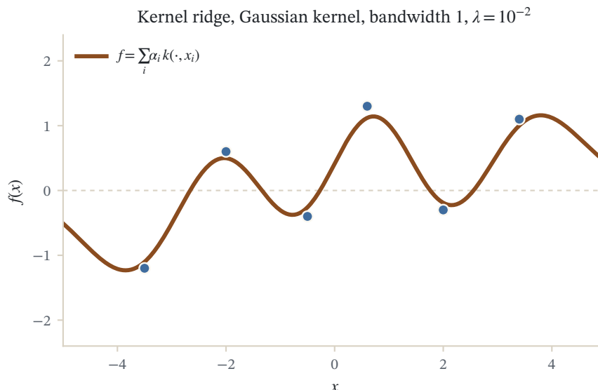
Figure 3.2: Kernel ridge regression on six points with a Gaussian kernel (bandwidth 1, ridge \lambda = 10^{-2} ). The curve is the exact solution f = \sum_i \alpha_i k(\cdot, x_i) with \alpha = (K + \lambda nI)^{-1}y .
