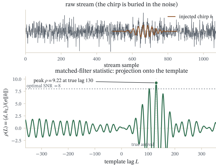
Figure 57.2: Matched filtering as a noise-weighted inner product: correlating a template against noisy data peaks sharply at the true lag, the optimal linear detector for a known signal in coloured noise.
