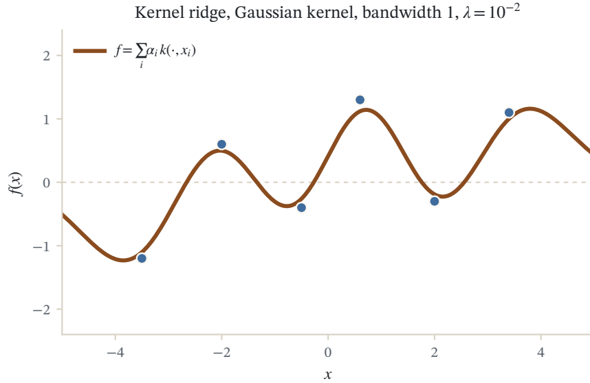
Figure 5.1: Kernel ridge regression on six points with a Gaussian kernel (bandwidth 1, ridge \lambda = 10^{-2} ). The curve is the exact solution f = \sum_i \alpha_i k(\cdot, x_i) with \alpha = (K + \lambda nI)^{-1}y .
