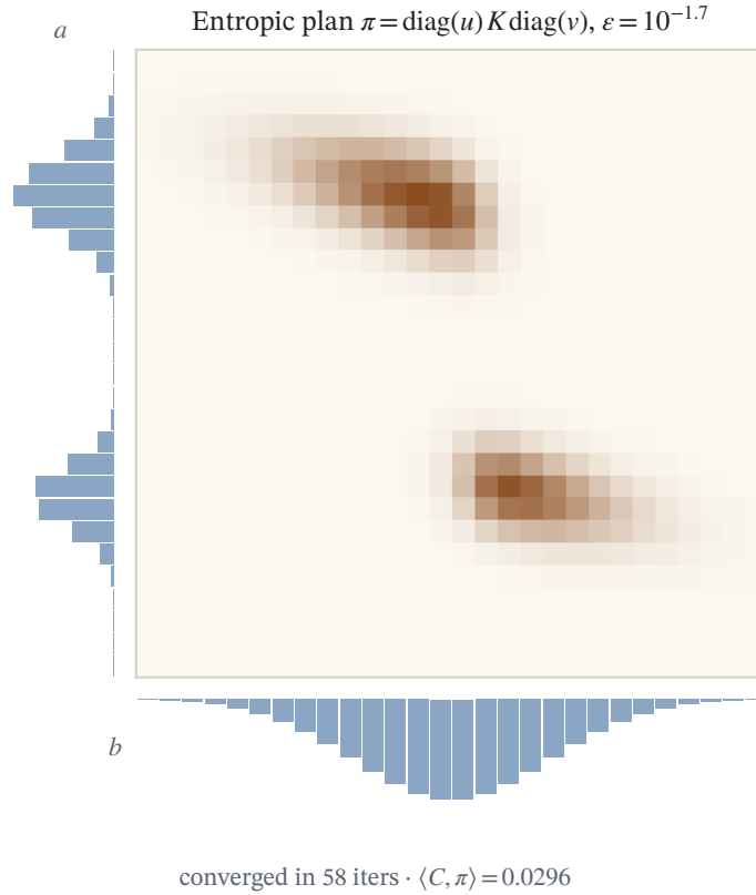
Figure 32.1: The entropic optimal-transport plan \pi = \text{diag}(u)K \text{diag}(v) between a two-bump source and a wide target, converged by alternating Sinkhorn normalizations u \leftarrow a \oslash (Kv) , v \leftarrow b \oslash (K^\top u) .
