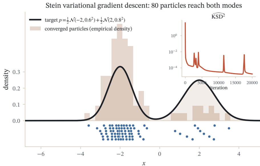
Figure 35.1: Stein variational gradient descent transports particles toward the two-mode target p = \frac{1}{2}\mathcal{N}(-2, 0.6^2) + \frac{1}{2}\mathcal{N}(2, 0.8^2) . The two terms \frac{1}{2}\mathcal{N}(-2, 0.6^2) and \frac{1}{2}\mathcal{N}(2, 0.8^2) are both modes of the target, pushing particles toward regions of high density. The driving force k(x_j, x_i) s_p(x_j) is a both modes and average of the modes, pushing particles toward regions of high density. The repulsion \nabla_{x_j} k(x_j, x_i) points particles away from one another, and without it every particle would collapse onto the same mode. Their balance is what makes the particles spread out into the shape of p rather than piling up at its peak. Both terms use only s_p , so SVGD samples an unnormalized posterior with no MCMC and no normalizer, which is why it reappears in Bayesian inference as a fast deterministic alternative to sampling.
