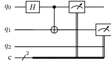
Fig. 6. Temporal Bell Pairs experiment circuit generating entanglement between Qubit 0 and Qubit 1.
