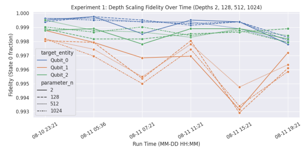
Fig. 3. Depth Scaling Fidelity Over Time (Depths 2, 128, 512, 1024)
