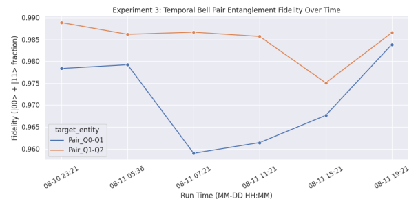
Fig. 7. Temporal Bell Pair Entanglement Fidelity Over Time
