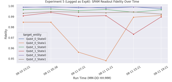
Fig. 11. SPAM Readout Fidelity Over Time
