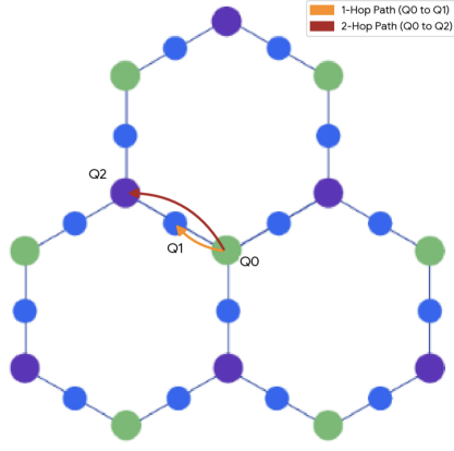
Fig. 12. Routing on Heavy-Hex Lattice (1-hop vs. 2-hop)
