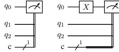
Fig. 10. State Preparation and Measurement (SPAM) circuits for Qubit 0. The left circuit measures the default |0\rangle ground state, while the right circuit applies a Pauli-X gate to prepare and measure the |1\rangle excited state.
