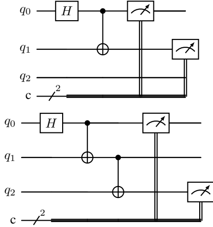
Fig. 13. Path Distance routing fidelity circuits. The top circuit evaluates a standard 1-hop entanglement path directly between adjacent qubits ( Q_0 and Q_1 ). The bottom circuit evaluates a 2-hop path by extending the entanglement to Q_2 before measuring the terminal endpoints ( Q_0 and Q_2 ).
