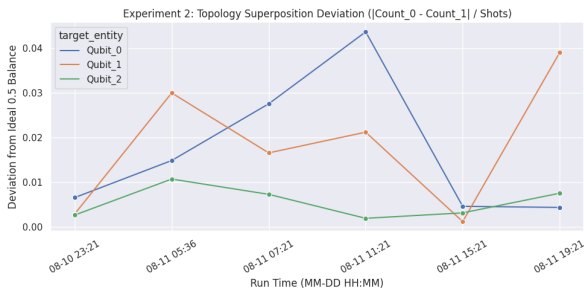
Fig. 5. Topology Superposition Deviation ( \frac{|Count_0 - Count_1|}{Shots} )
