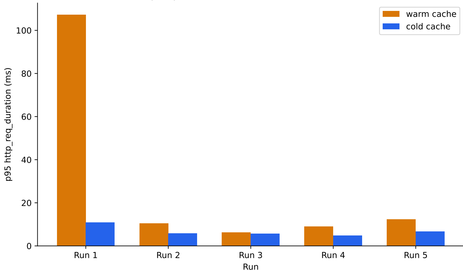
p95 per run - warm cache vs cold cache
