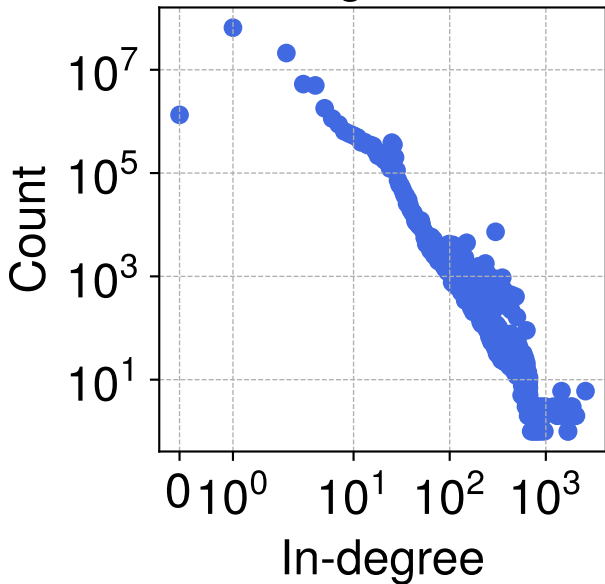
Payment Graph 11 in-degree dist.
