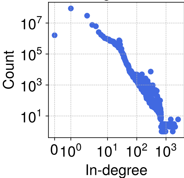
Payment Graph 12 in-degree dist.
