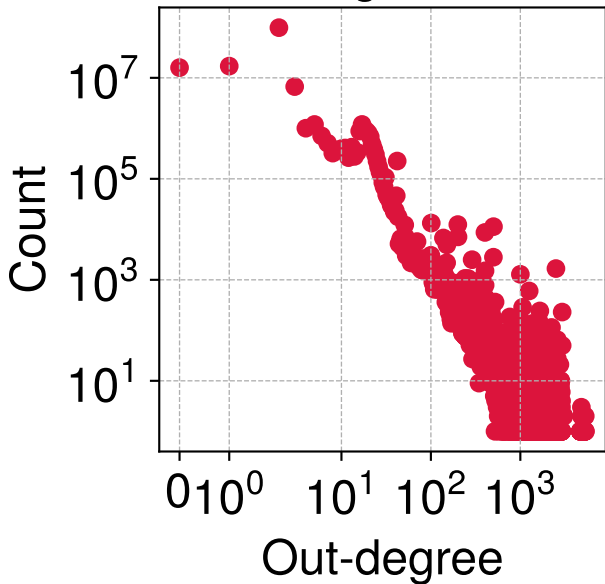
Payment Graph 12 out-degree dist.
