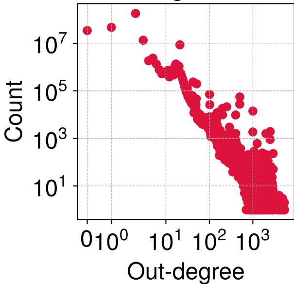
Payment Graph 14 out-degree dist.
