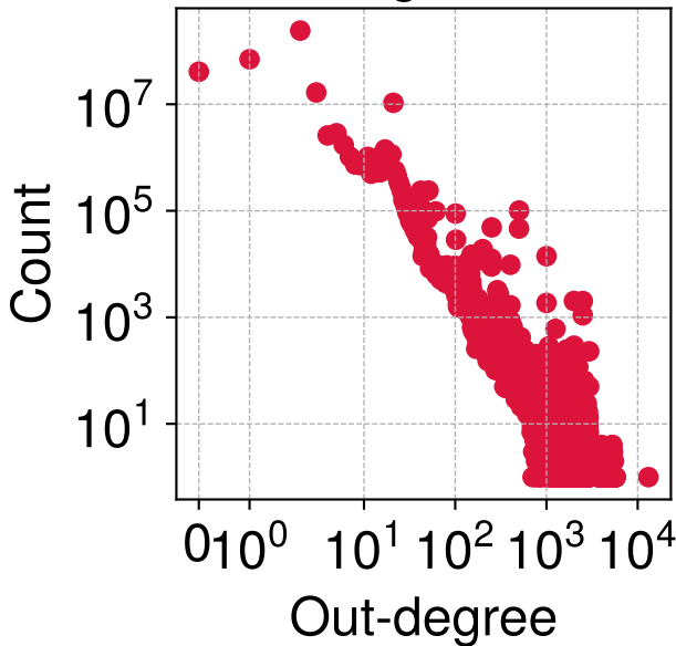
Payment Graph 15 out-degree dist.
