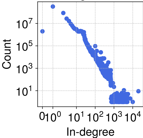
Payment Graph 16 in-degree dist.
