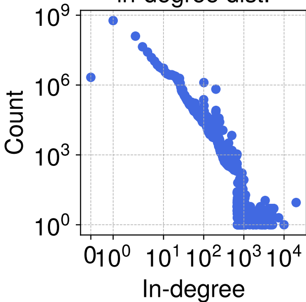
Payment Graph 19 in-degree dist.
