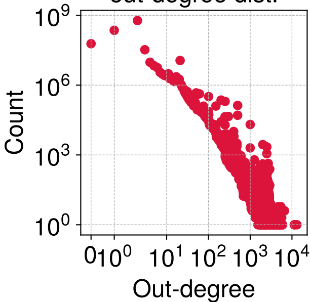
Payment Graph 20 out-degree dist.
