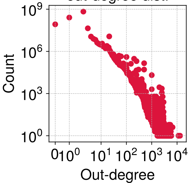
Payment Graph 21 out-degree dist.
