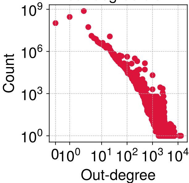
Payment Graph 22 out-degree dist.
