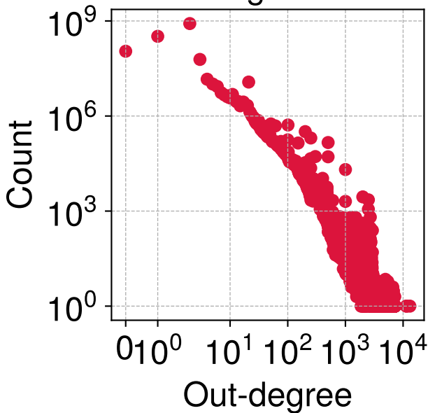
Payment Graph 23 out-degree dist.
