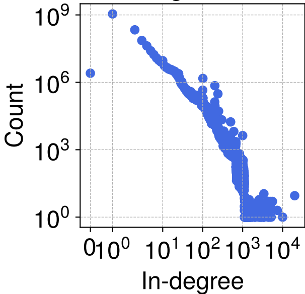
Payment Graph 24 in-degree dist.
