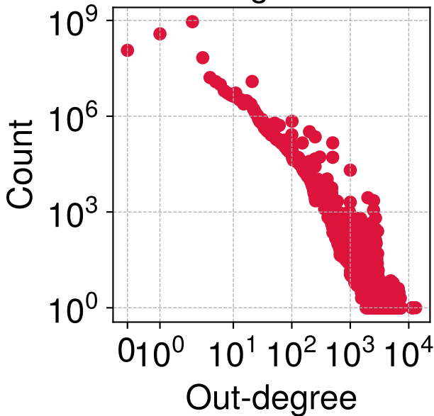
Payment Graph 24 out-degree dist.
