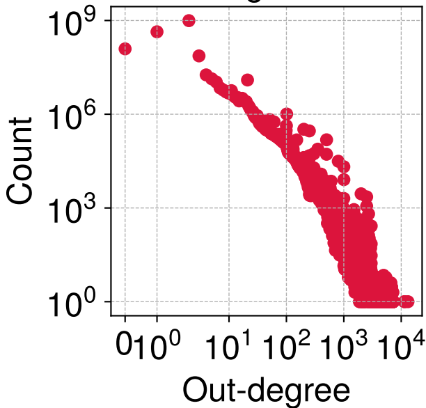
Payment Graph 25 out-degree dist.
