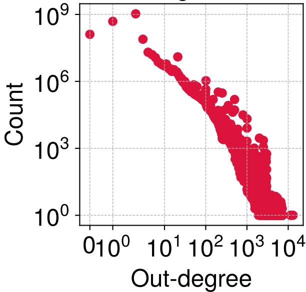
Payment Graph 26 out-degree dist.
