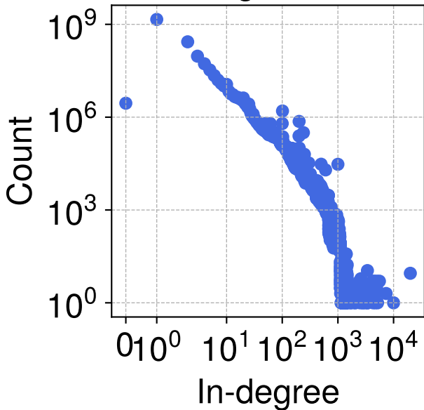
Payment Graph 27 in-degree dist.
