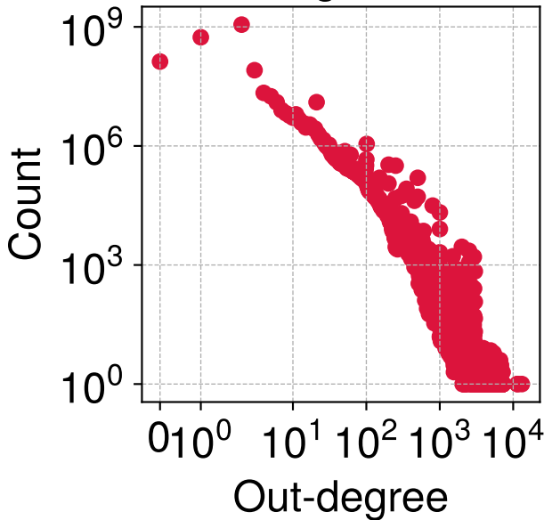
Payment Graph 27 out-degree dist.
