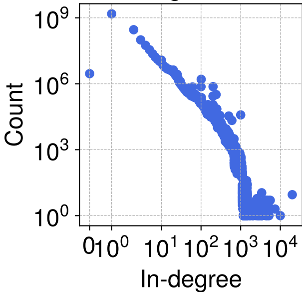
Payment Graph 28 in-degree dist.
