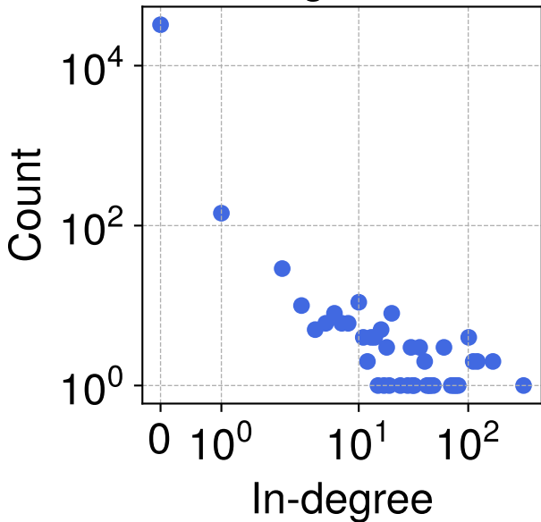
Payment Graph 2 in-degree dist.
